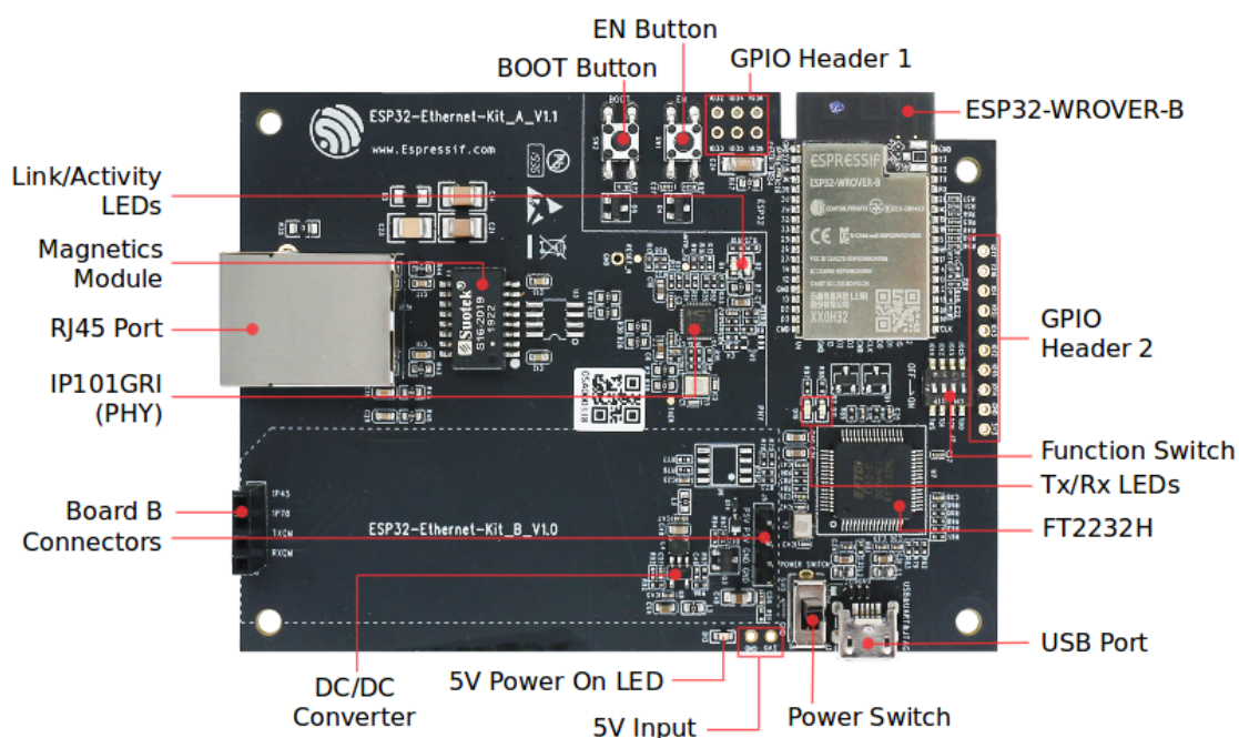
Fig. 14: ESP32-Ethernet-Kit - Ethernet board (A) layout (click to enlarge)
