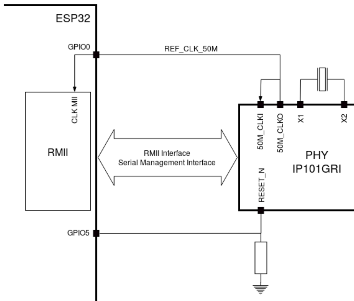
Fig. 16: RII Clock from IP101GRI PHY (click to enlarge)
