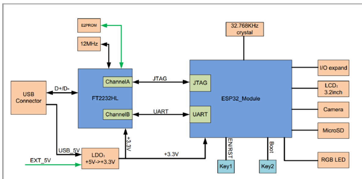
Fig. 26: ESP-WROVER-KIT block diagram
