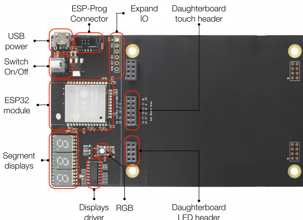
Fig. 8: Motherboard Components
